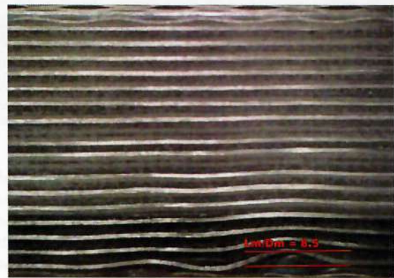
Figure 7 – Correct measurement of the wrinkle severity figure when more than one wrinkle is present
