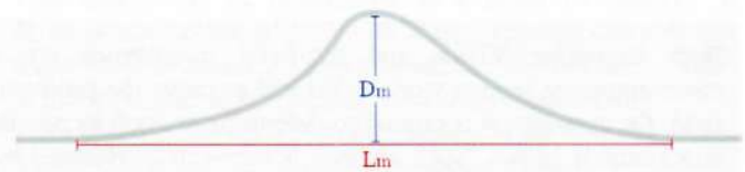
Figure 1 – Dimensions of a wrinkled ply
